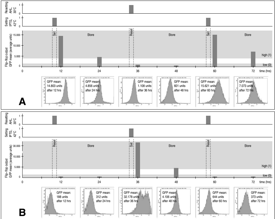
Fig. 4. Inducer-dependent switching. Repeated activation and deactivation of the toggle switch based on inducers and temperature. Temperature was switched every 24 hours. Cells were incubated with inducers for 12 hours, followed by growth for 12 hours without inducers, initially kept at 30°C (A) and 42°C (B). The cells successfully switched states thrice.
