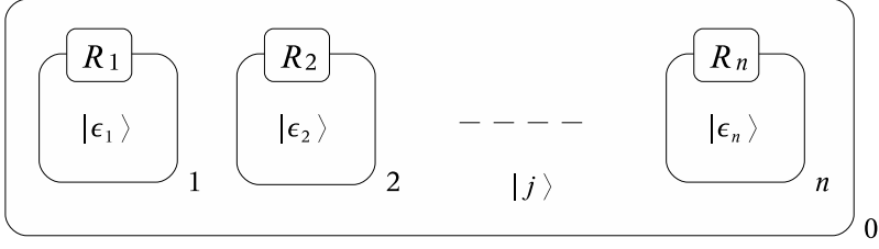
Fig. 1. A configuration of the simulating P system
