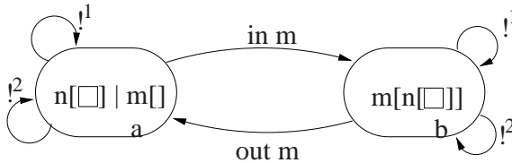
Fig. 1. A labeled transition system for the process n[!^1 \text{in } m. !^2 \text{out } m] \mid m[ ]
