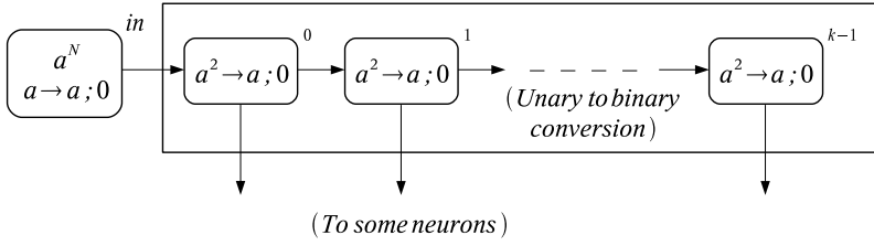
Fig. 4. A maximally parallel SN P system that converts a unary encoded positive integer number to binary form
