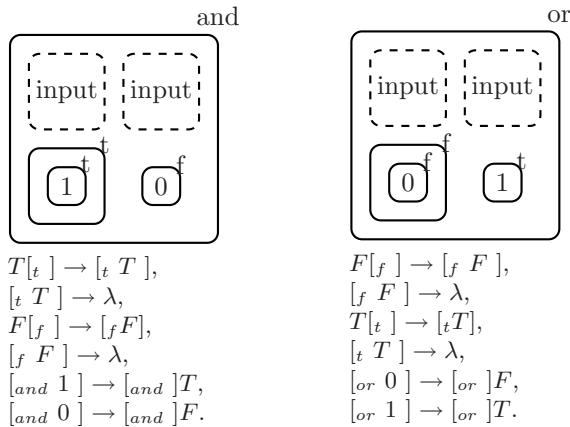
Fig. 1. AND and OR gadgets which can be nested together to simulate a circuit. The input is either a T, F, or a nested series of gadget membranes. A NOT gate membrane can be made with the rules [not \ T] \rightarrow [not \ ]F , [not \ F] \rightarrow [not \ ]T .
