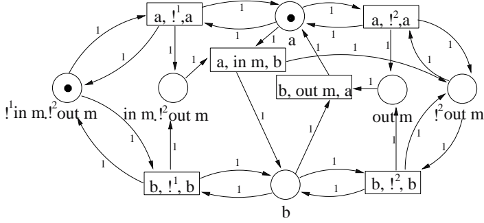
Fig. 3. The Petri net for the labeled process n[!^1 \text{ in } m. !^2 \text{ out } m] \mid m[ ]
