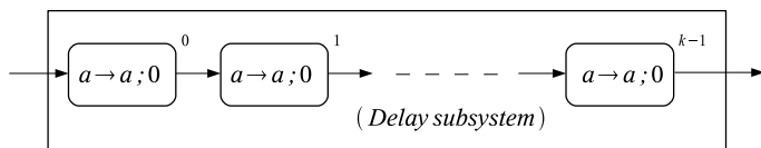
Fig. 6. An SN P system that delays of k steps the sequence of spikes given in input
