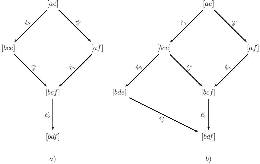
Fig. 7. Causal dependency and history causality
