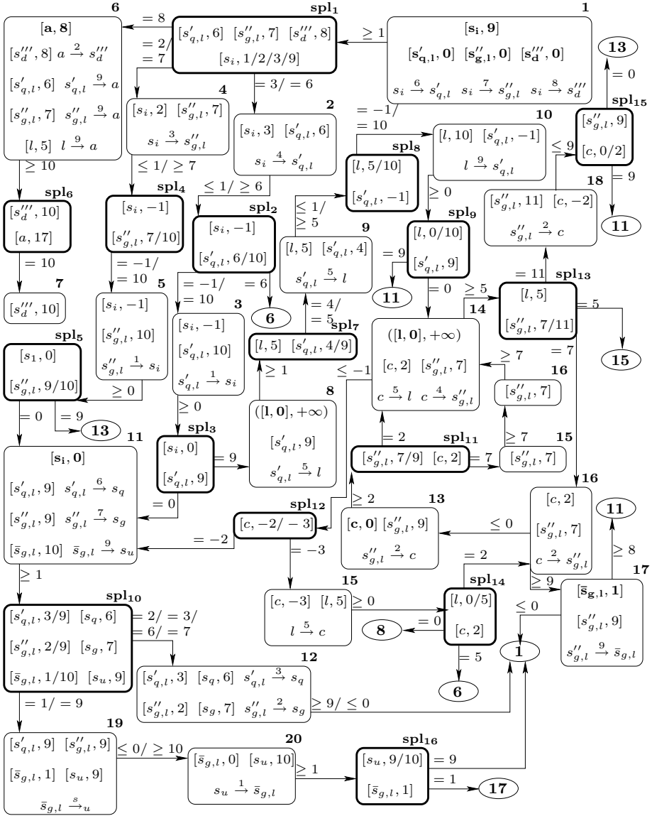
Fig. 2. The conformons-P system related to Theorem 1
