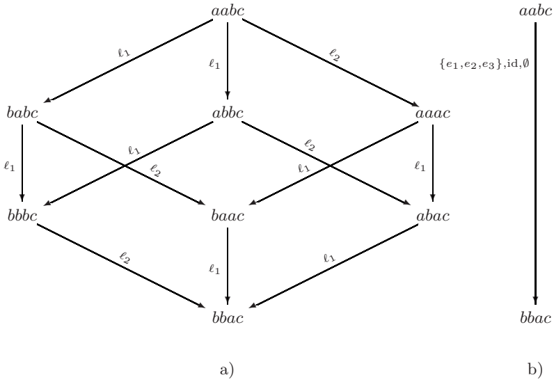
Fig. 2. A lts corresponding to abc \xrightarrow{mgr} bbac
