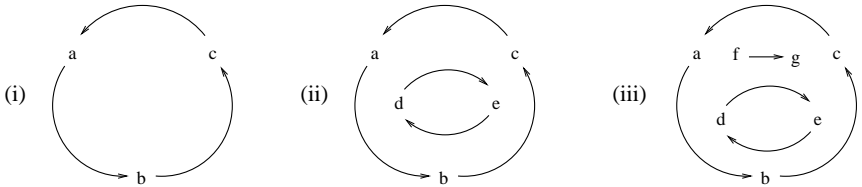
Fig. 1. (i) represents (a \cdot b \cdot c)^L ; (ii) represents (a \cdot b \cdot c)^L \mid (d \cdot e)^L ; (iii) represents (a \cdot b \cdot c)^L \mid ((d \cdot e)^L \mid f \cdot g) .
